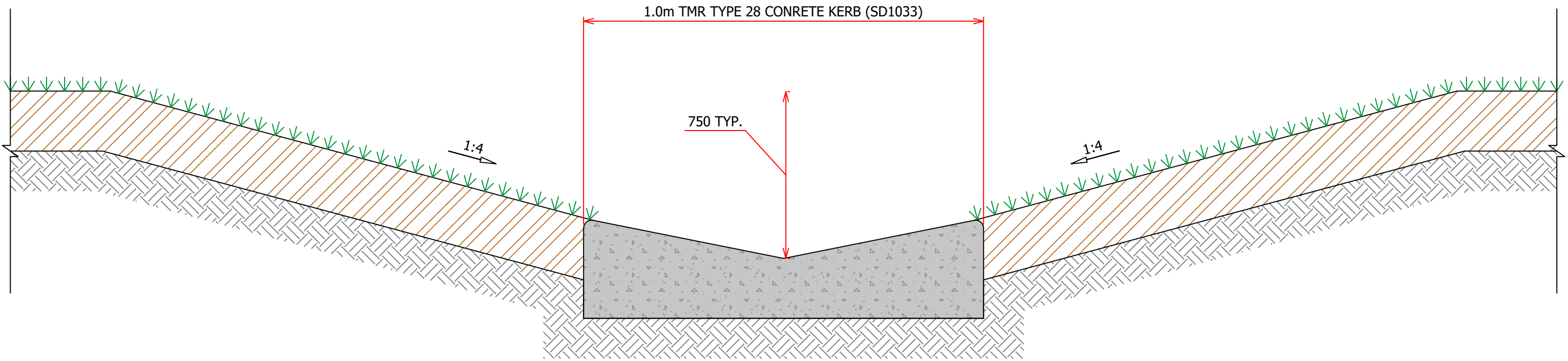
GRASSED SWALE WITH SPOON DRAIN TYPICAL DETAIL N.T.S
