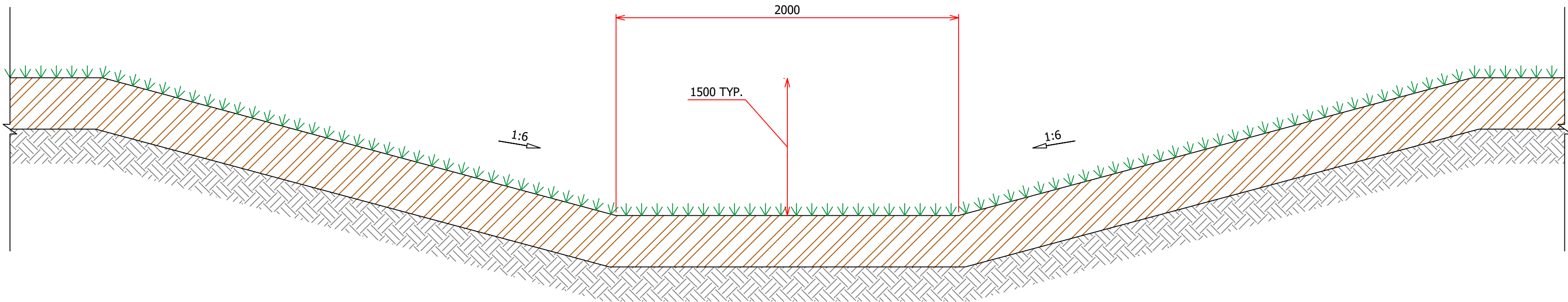
VEGETATED SWALE TYPICAL DETAIL N.T.S
