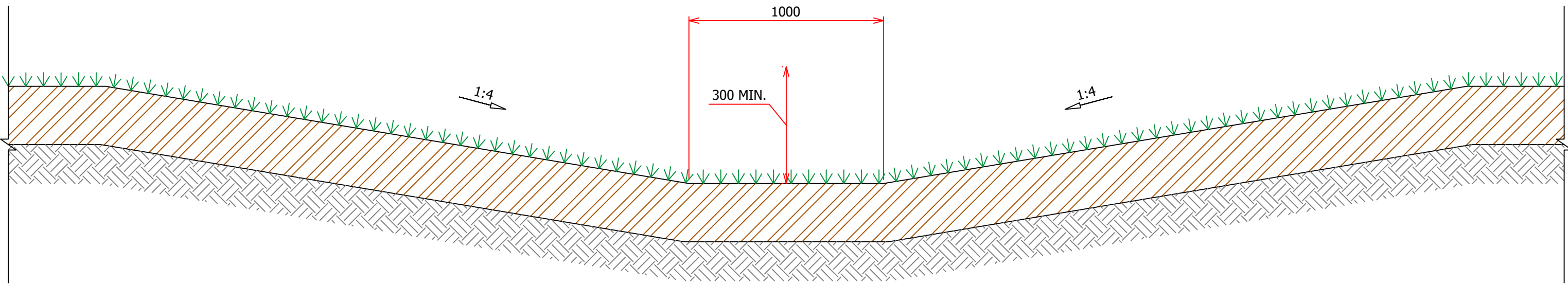
GRASSED SWALE TYPICAL DETAIL N.T.S
